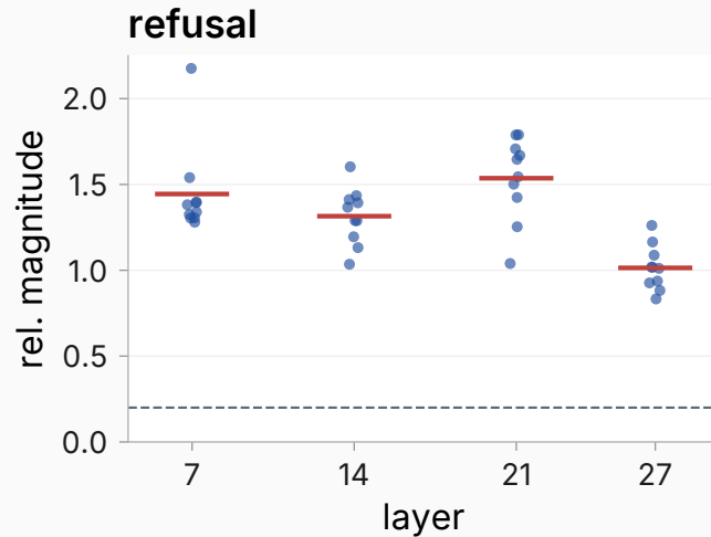
Per-context relative magnitude of Delta(C,b) by layer (instruct, 10 contexts)
