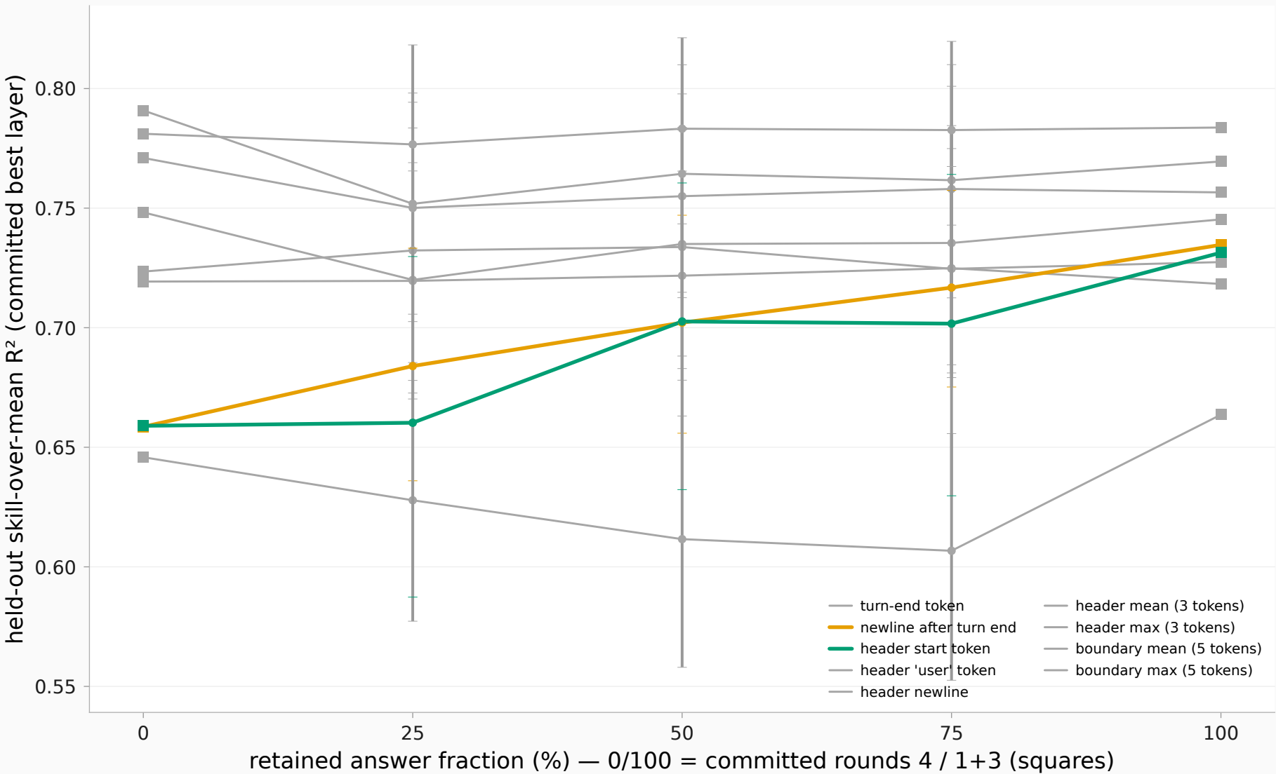
Dose trace: predicting each boundary summary as the answer is truncated
