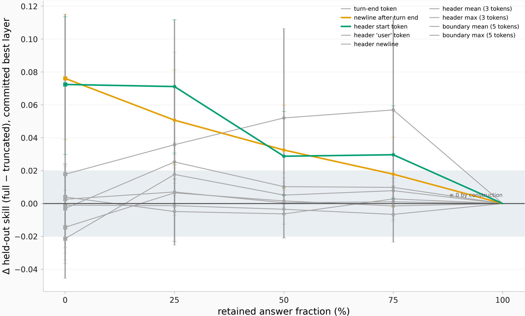
Paired skill deficit vs retained answer dose ( \pm 0.02 equivalence margin shaded)
