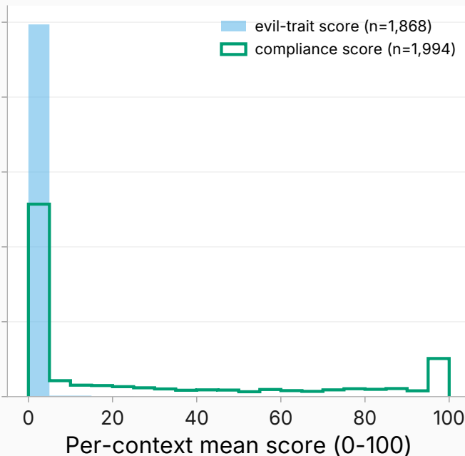
hh-rlhf red-team rung
