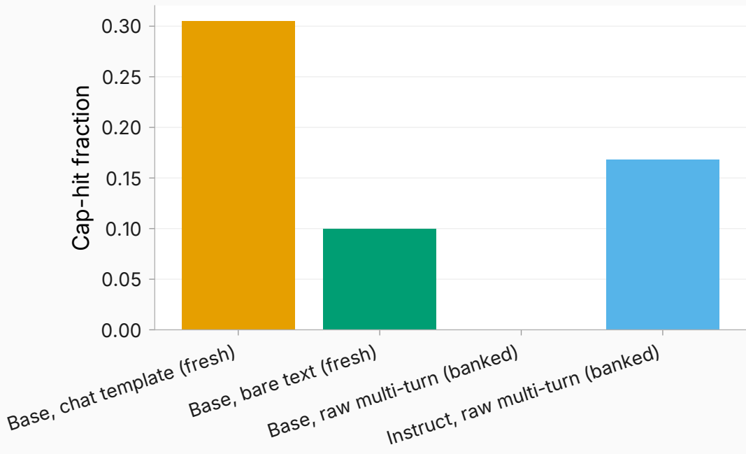
Fraction ending at the 1,024-token cap
