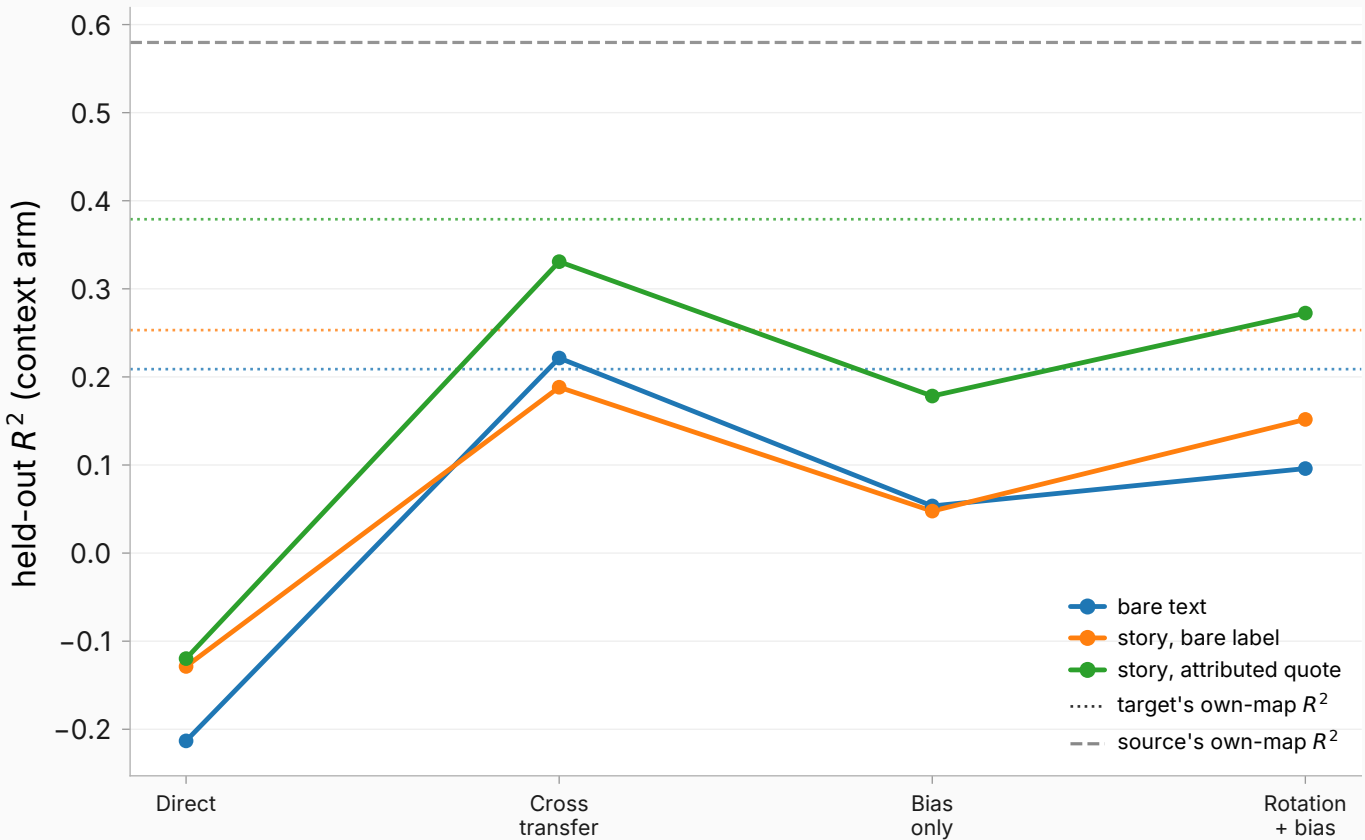
Transferring the assistant's chat-template map to other framings (on-policy, instruct)
