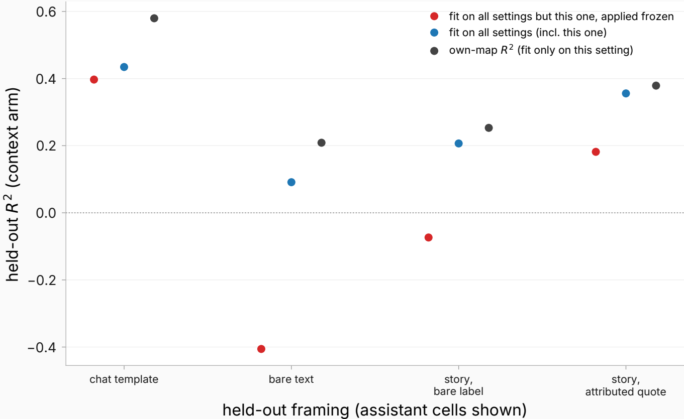
Map fit on all framings but one, applied to the held-out framing (on-policy, instruct)
