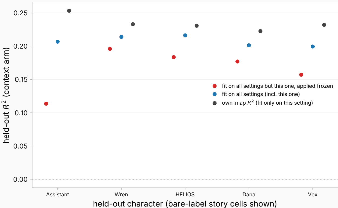
Map fit on all characters but one, applied to the held-out character (on-policy, instruct)
