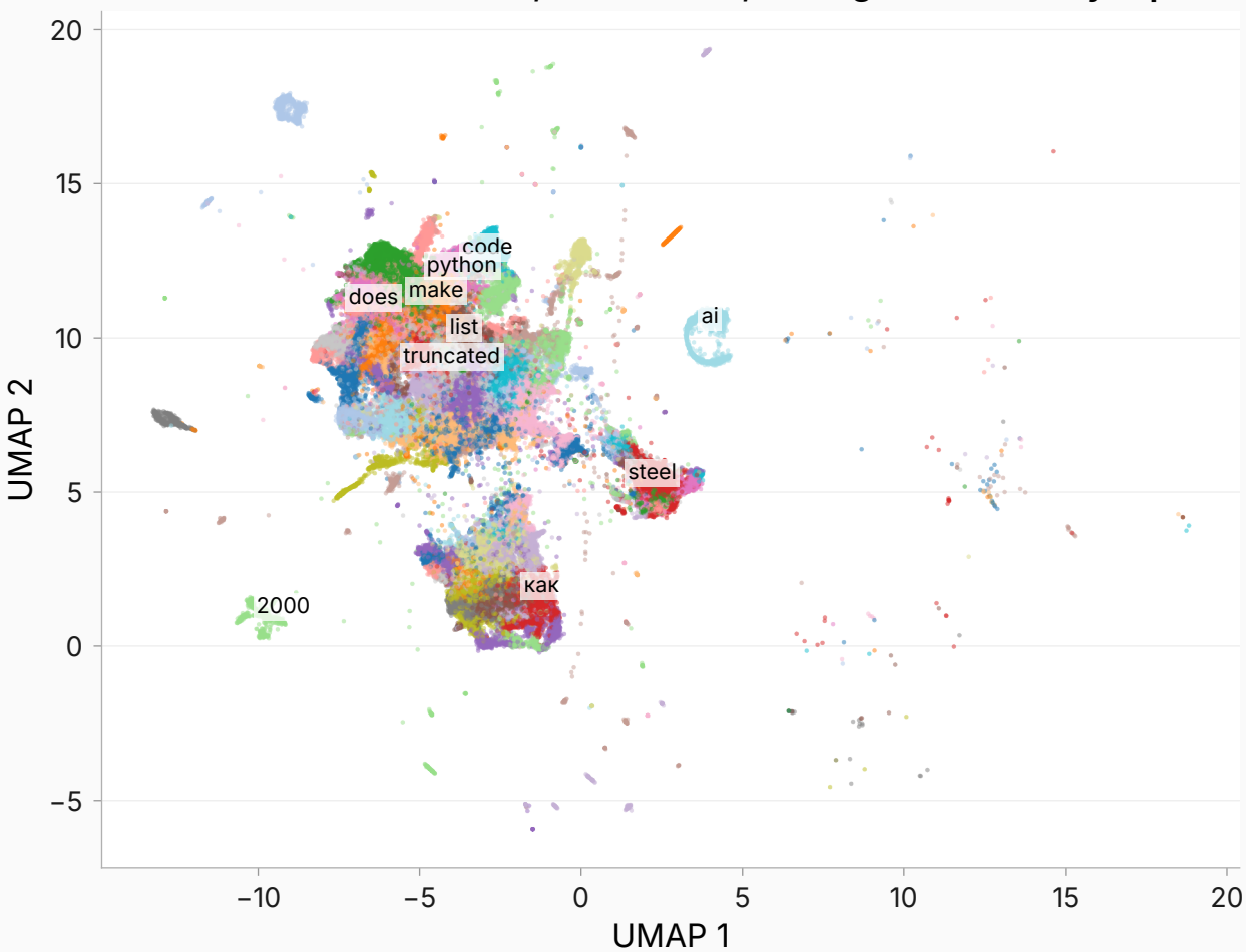
context clusters (KMeans, 50 clusters; 10 largest labeled by top TF-IDF term)
