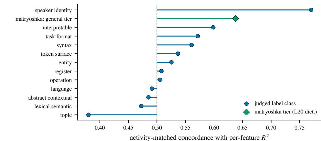
Figure 4. Concordance c (AUROC scale) between a feature’s class and its held-out R^2 , with pairs formed only within per-token firing-rate deciles so activity is matched, not just regressed out. 0.5 = \text{chance} . Circles: 12 judge-assigned classes over 120,716 features. Diamond: the matryoshka general tier a different dictionary and layer, so read its direction only, never its distance from the circles. No CIs exist for this statistic; gaps under \sim 0.02 are not readable.
