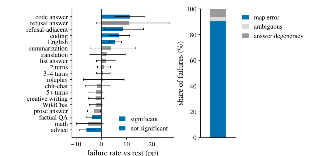
Figure 5. Retrieval failures against sampling-noise-free answer targets (each answer averaged over 5 on-policy draws), raw-euclidean read: n = 1,988 held-out contexts, pool 9,941, 180 failures, rank-1 0.909. Left: category failure rate minus the rest, 10,000-draw bootstrap CIs; significant = clears Benjamini–Hochberg FDR at q=0.05 . “Refusal answer” trends high but misses FDR ( n=30 ). Right: what the 180 misses are map error = the answer is still retrievable from a fresh draw of itself.
