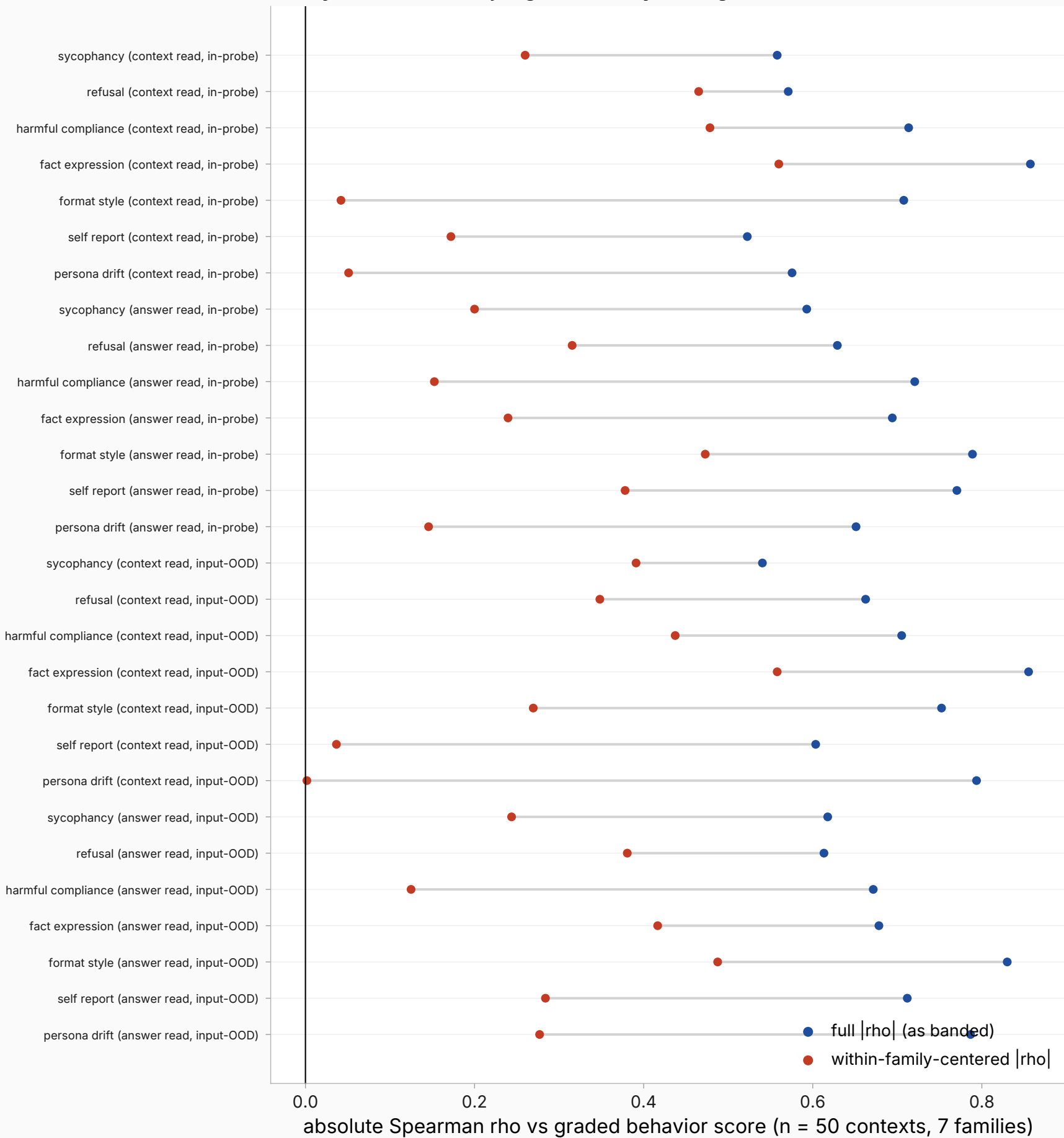
Behavior read-out at each best cell (27 of 28 clear their band): full vs family-centered rho (judge-reliability ceilings 0.68-0.96 bound attainable rho)
