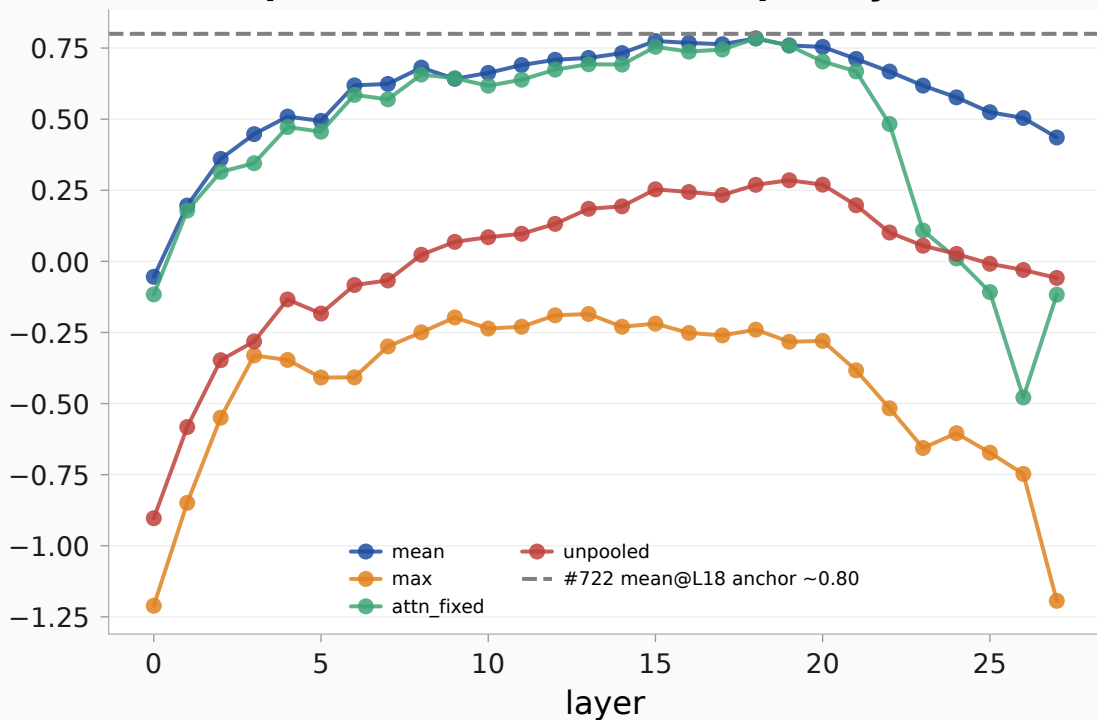
answer-profile reconstruction R^2 per layer (SECONDARY DV)
