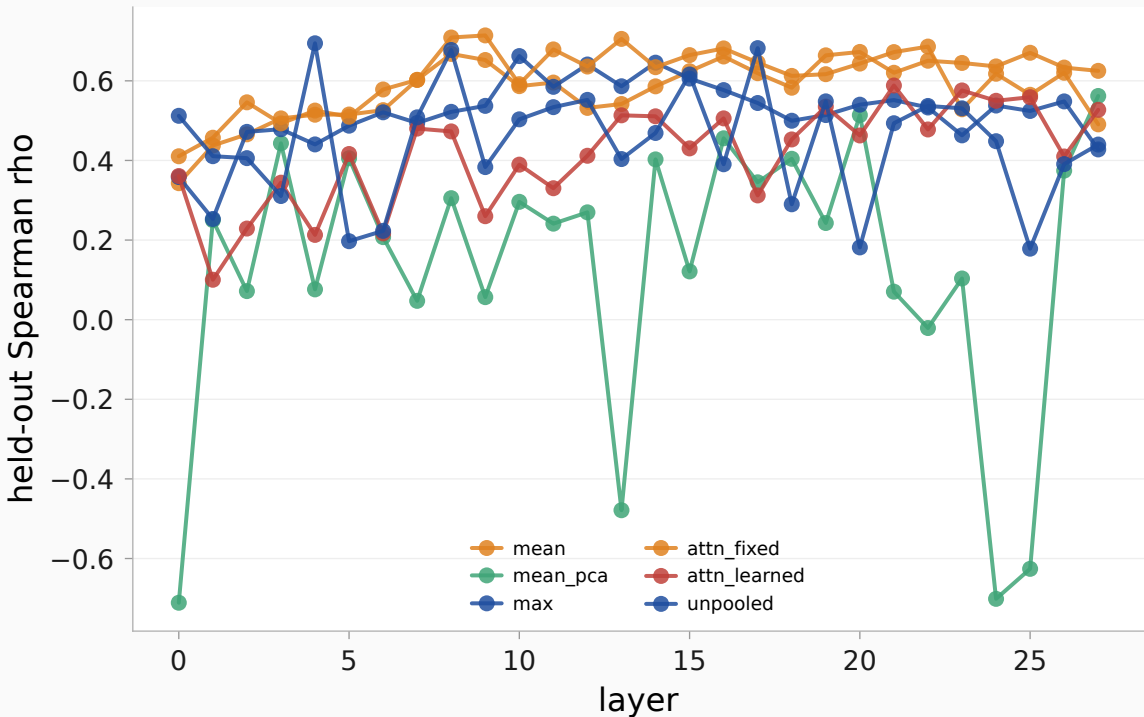
deception: pooling-operator E0-prediction rho per layer
