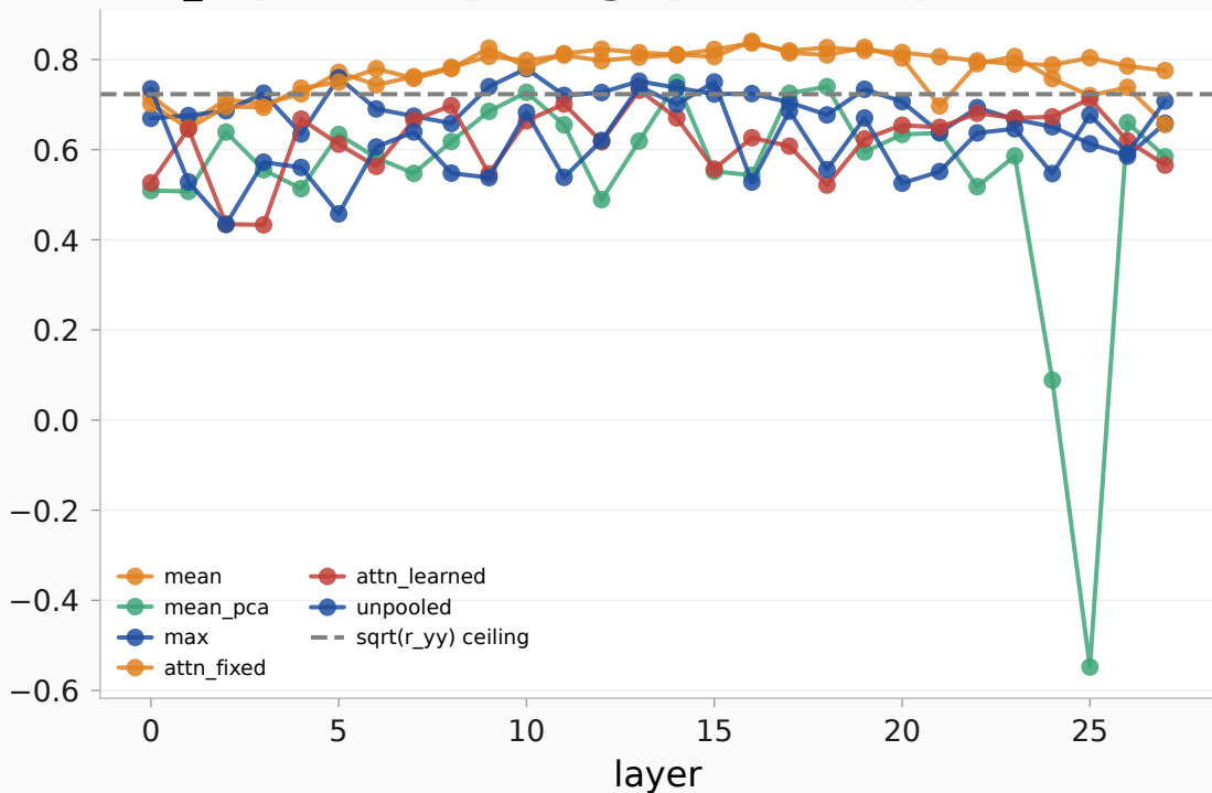
fact_expression: pooling-operator E0-prediction rho per layer
