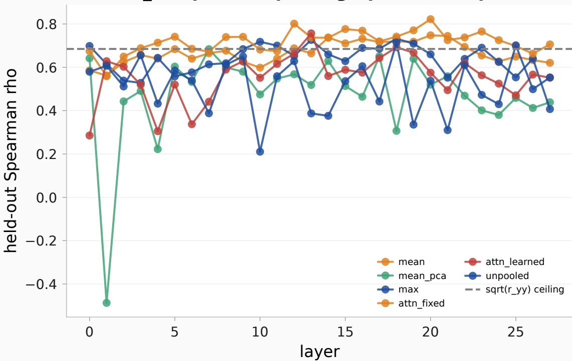
harmful_compliance: pooling-operator E0-prediction rho per layer
