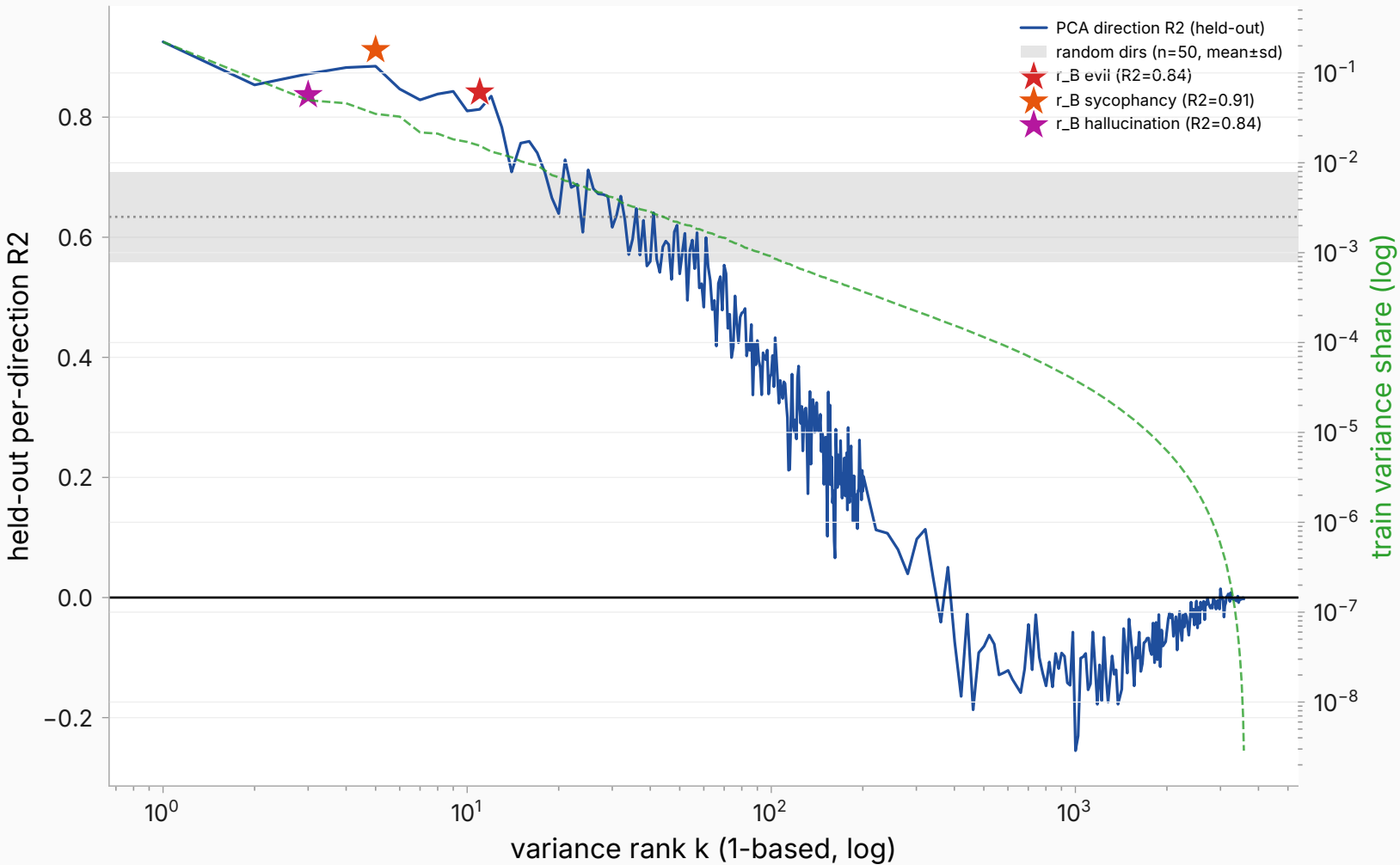
Per-direction predictability at L19 (best recon layer) — all 3 traits' r_B
