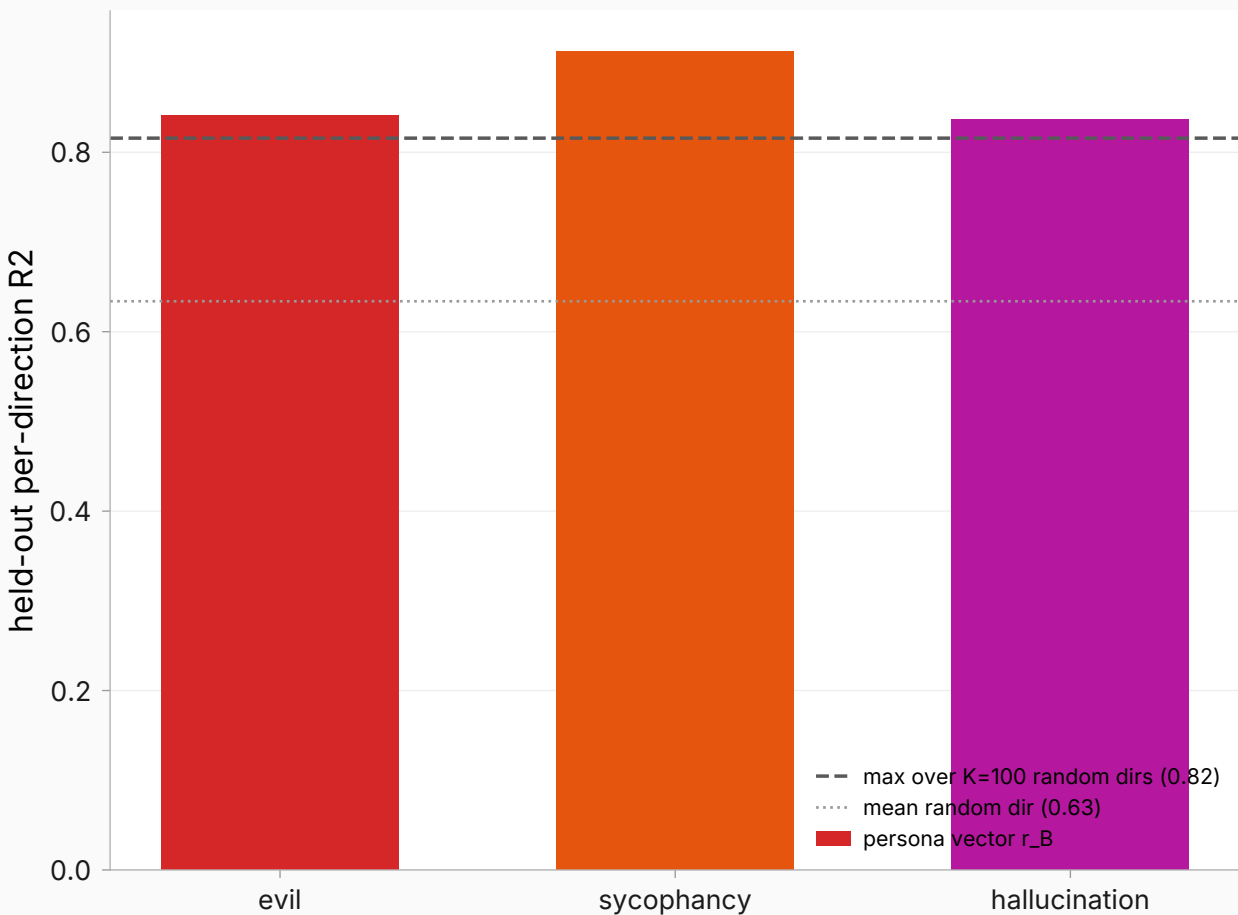
Persona vectors vs max-over-K random directions (L19)
