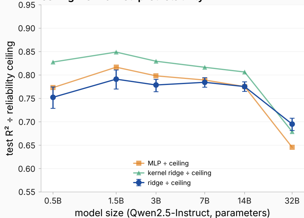
ceiling-normalized predictability
