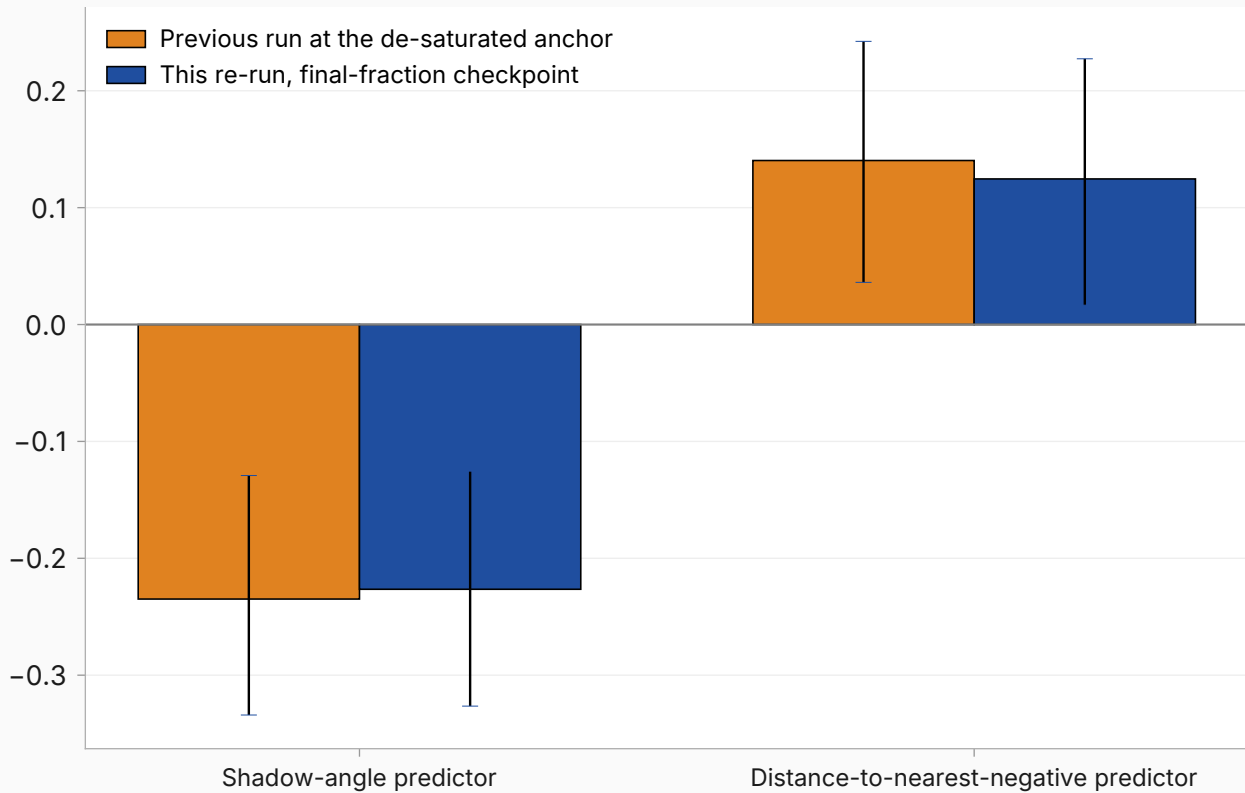
Partial Spearman correlation with held-out leakage
