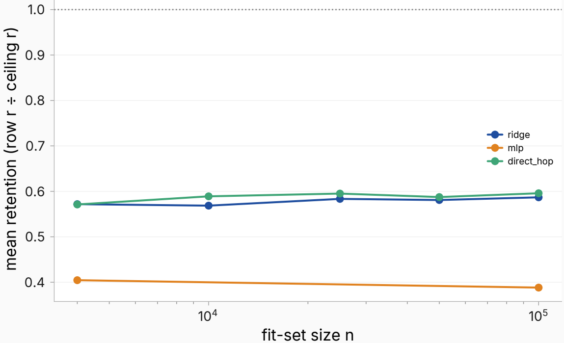
DV3 retention vs fit-set size (per class)
