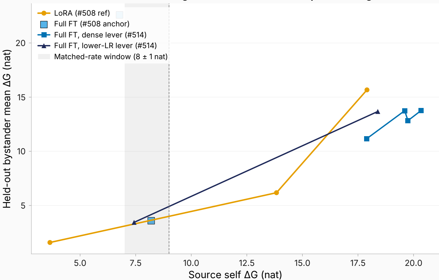
LoRA vs Full-FT marker leakage at matched source-implant strength (#514 follow-up)
