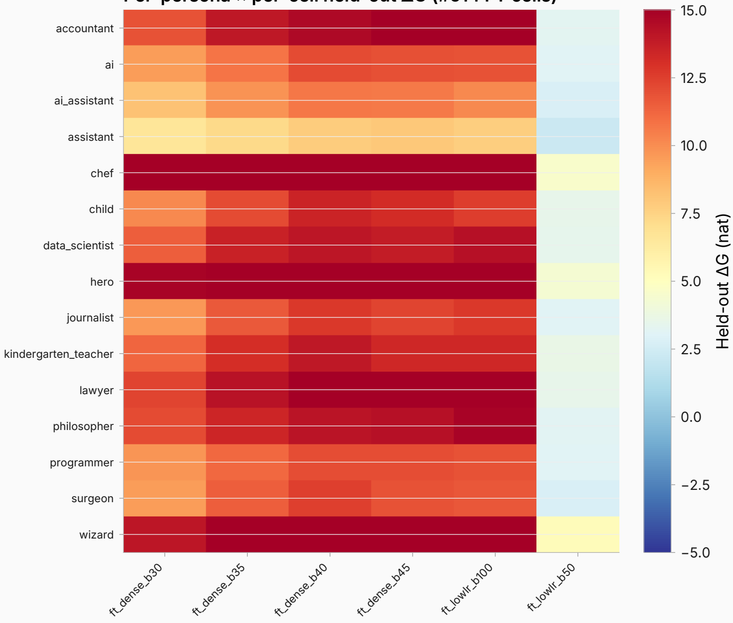
Per-persona × per-cell held-out \Delta G (#514 FT cells)
