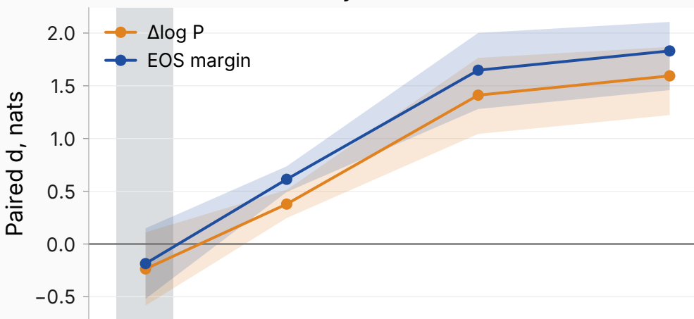
Wrong-persona probe — pirate (s18 shaded: band-adjacent read)
