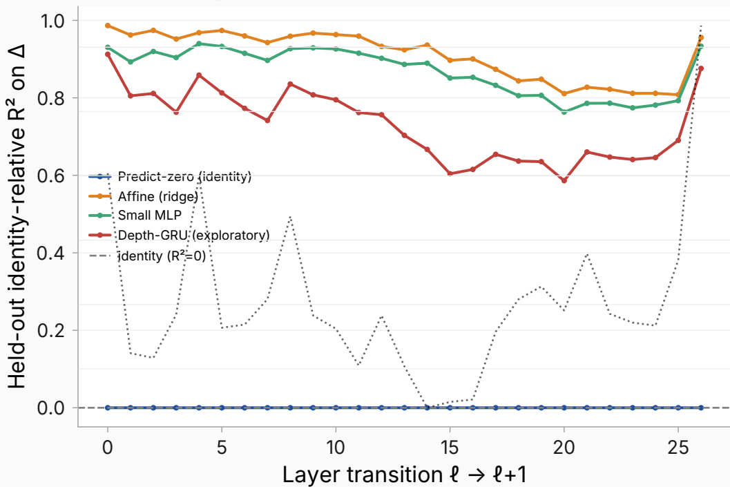
raw target space
