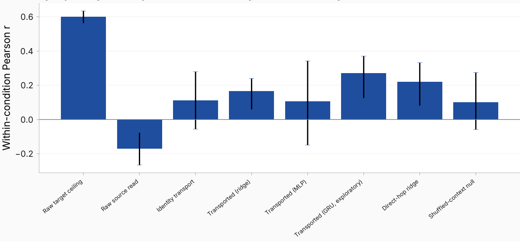
sycophancy — companion \ell^*=19 — many_shot (source layer 0)
