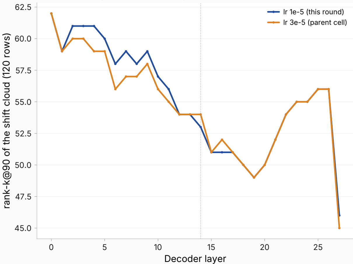
Own-text response arm: rank per layer
