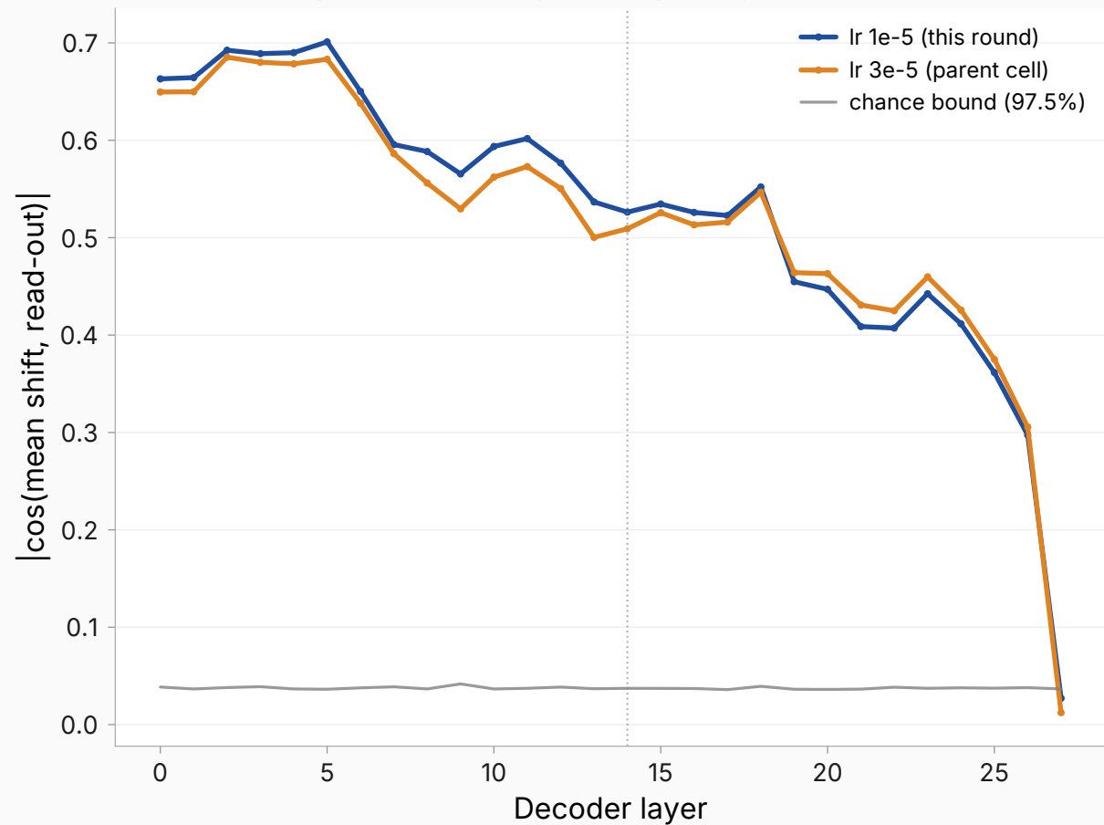
Own-text response arm: alignment per layer
