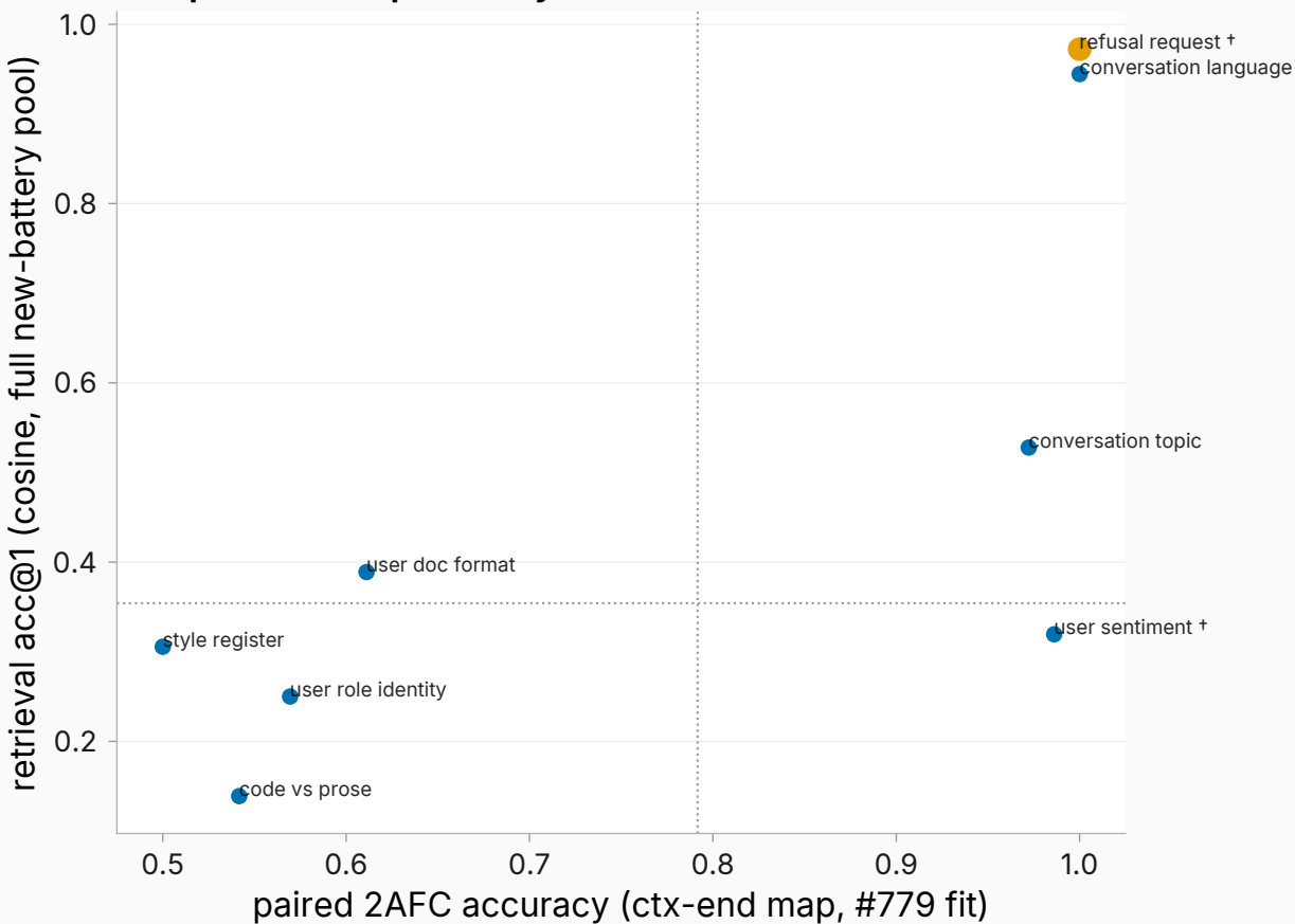
H3: pairwise separability vs exact retrieval — refusal rank 1/8 (2AFC), 1/8 (retrieval)
