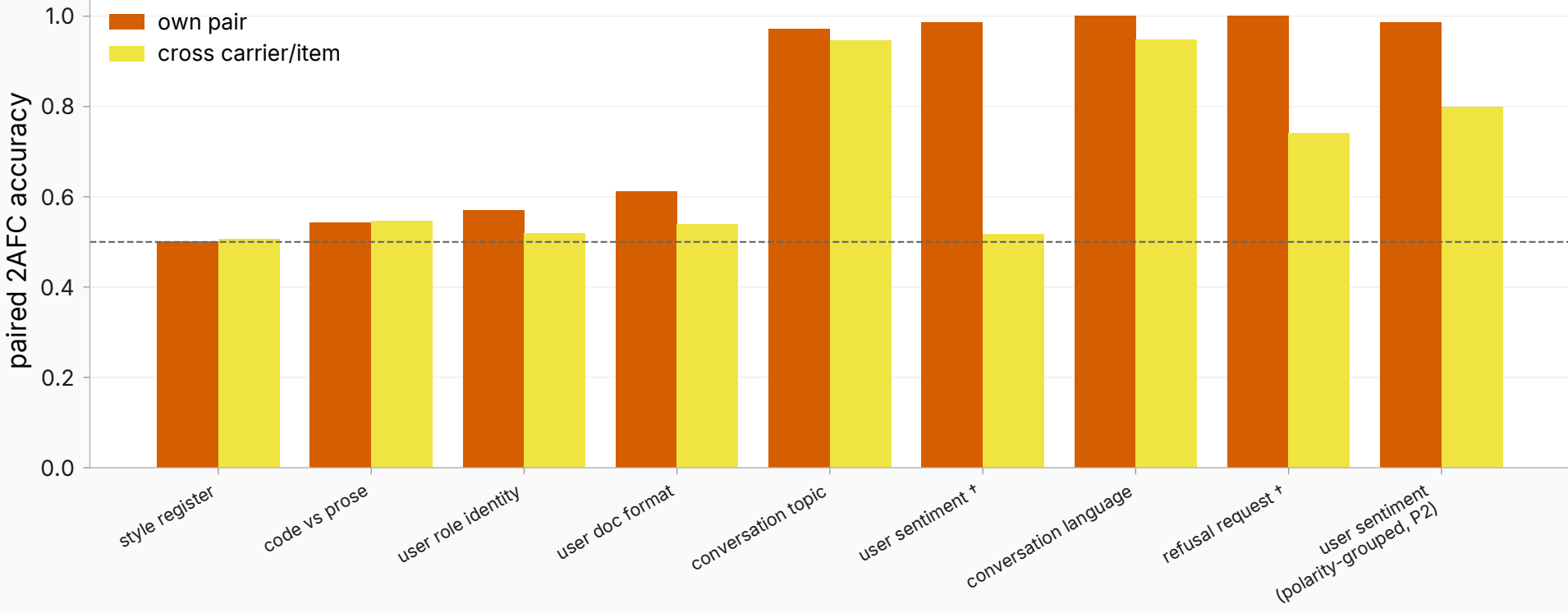
Carrier transfer: same value pair scored at other carriers (ctx-end map #779 fit, L19)
