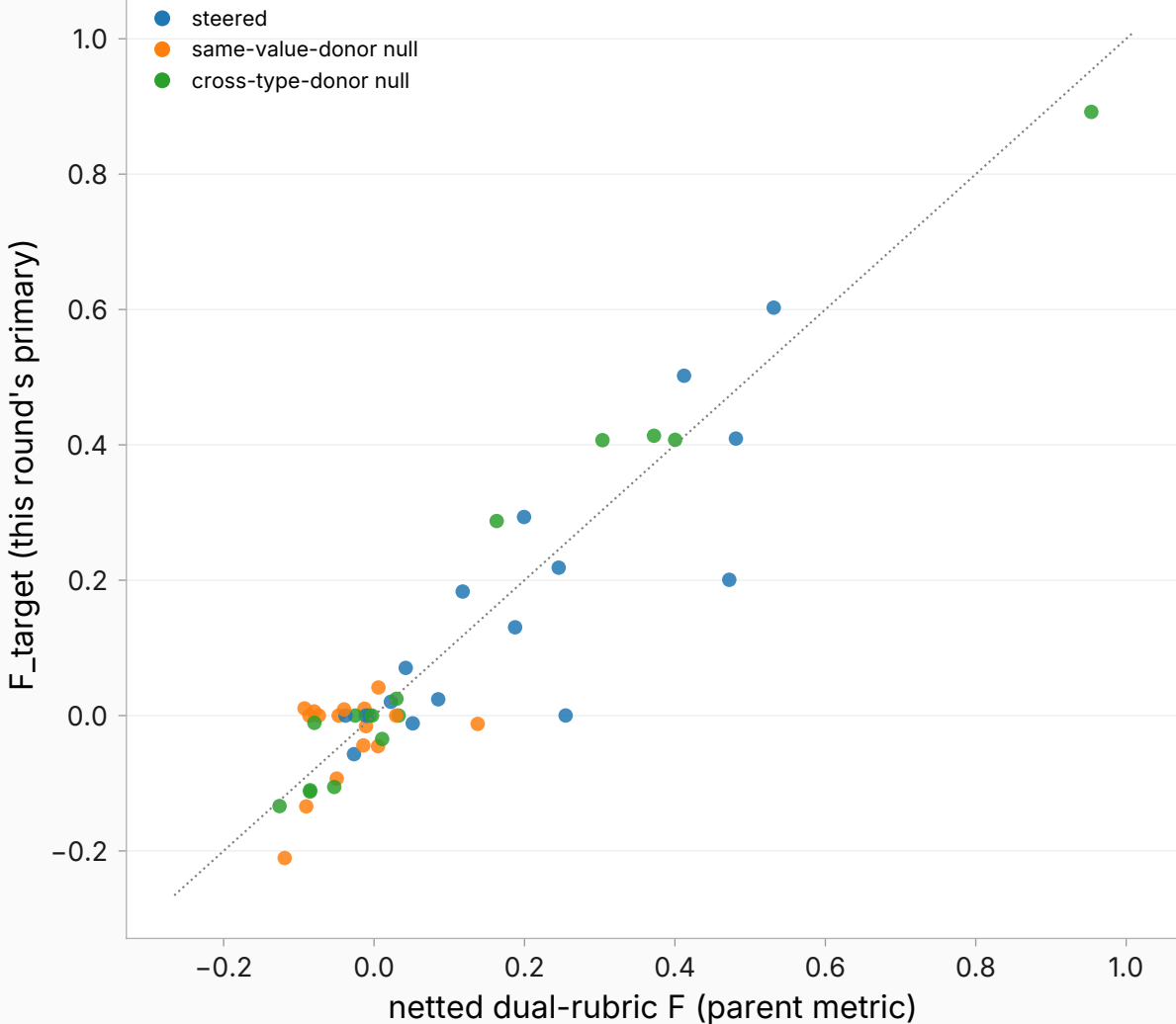
Netted dual-rubric F vs target-only F per (direction × slot × arm)
