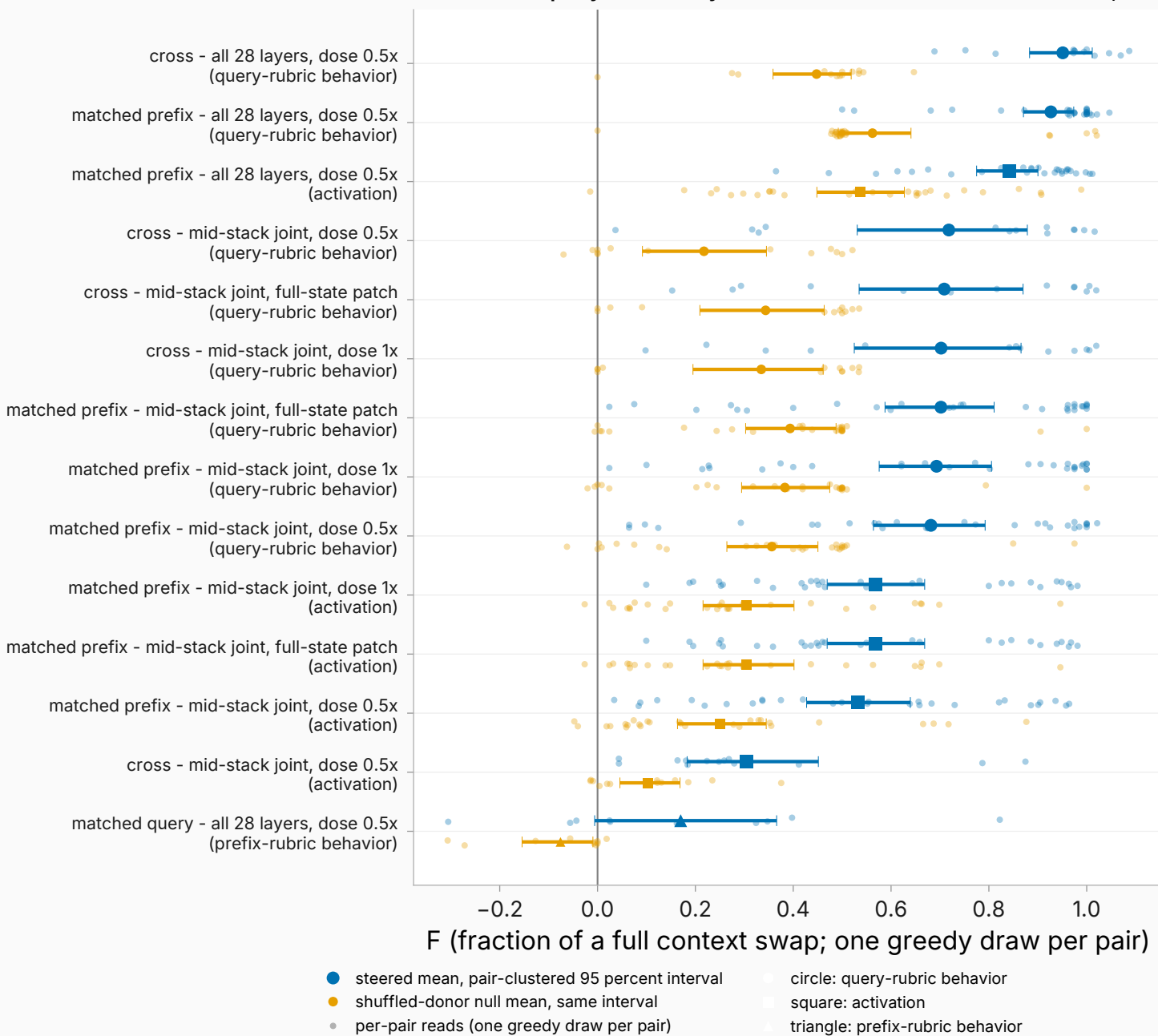
the 14 clean query-text family reads: steered vs shuffled-donor null, well-separated pairs
