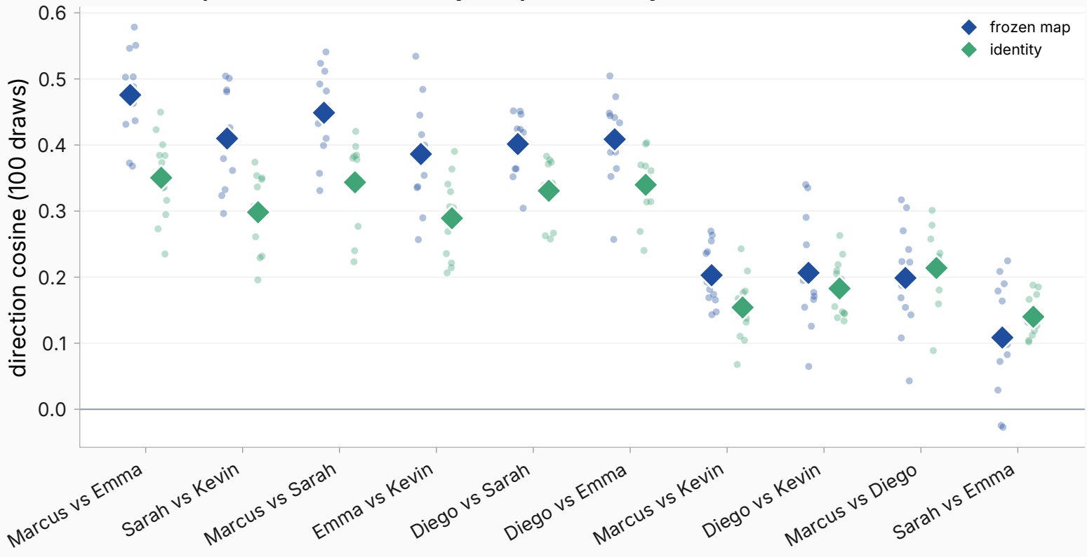
Per name-pair direction recovery: map vs identity
