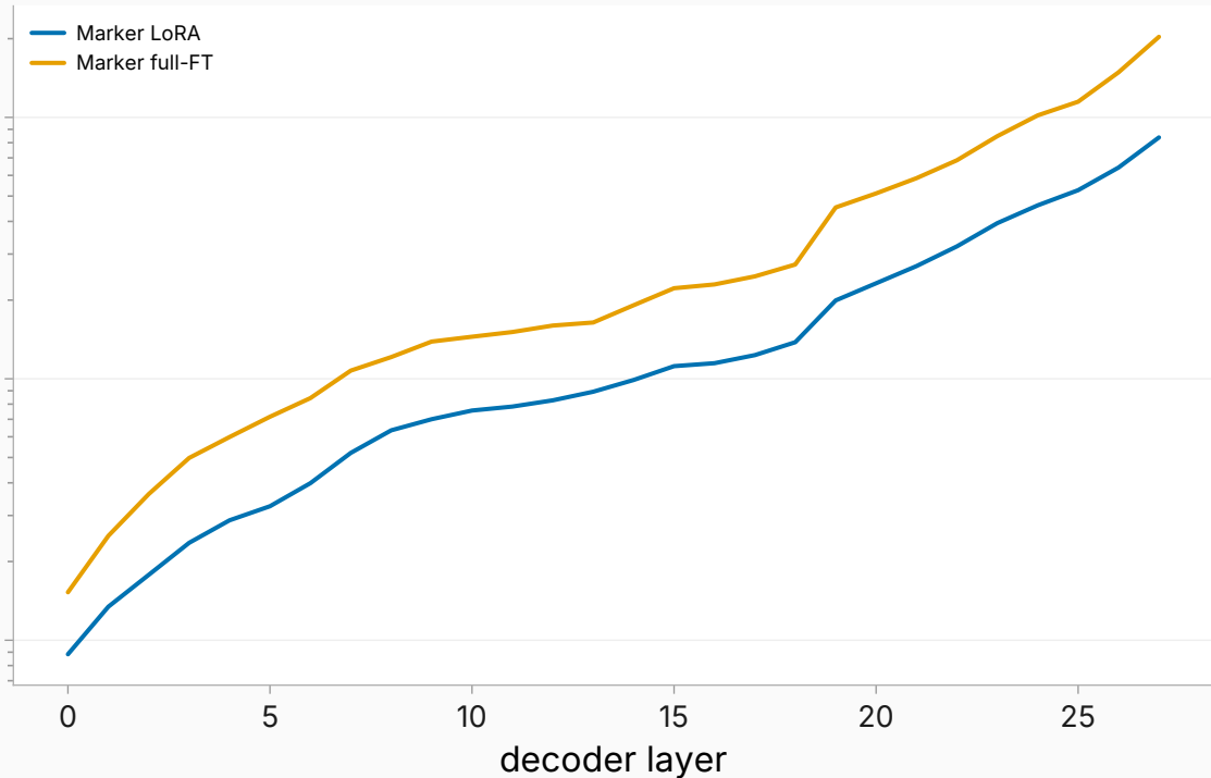
marker activation shift — response arm (selected checkpoint)
