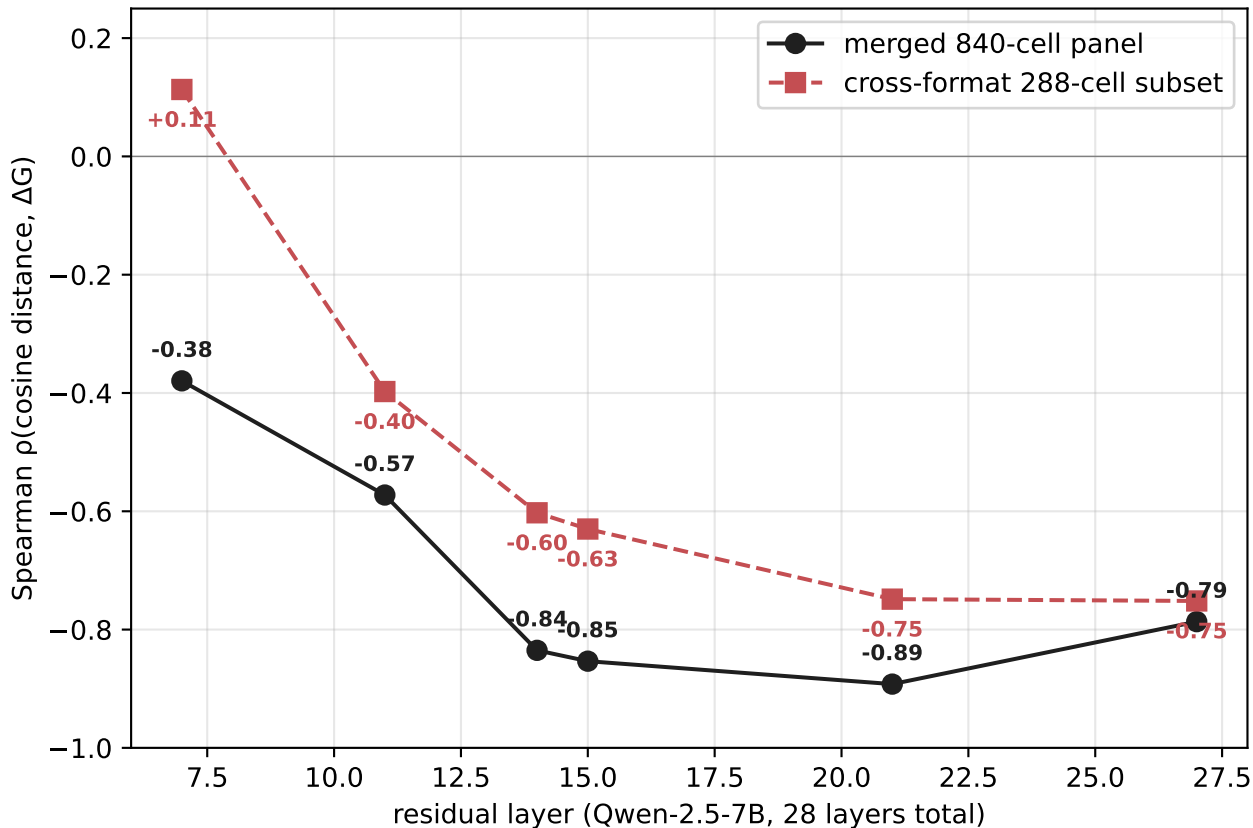
layer-sweep predictor strength
