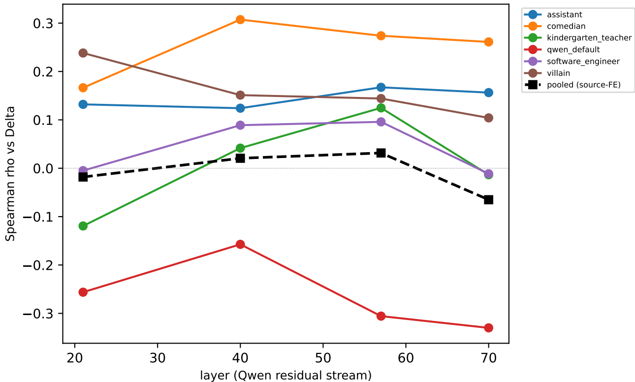
Cosine recipe (b) layer sweep — per-source rho
