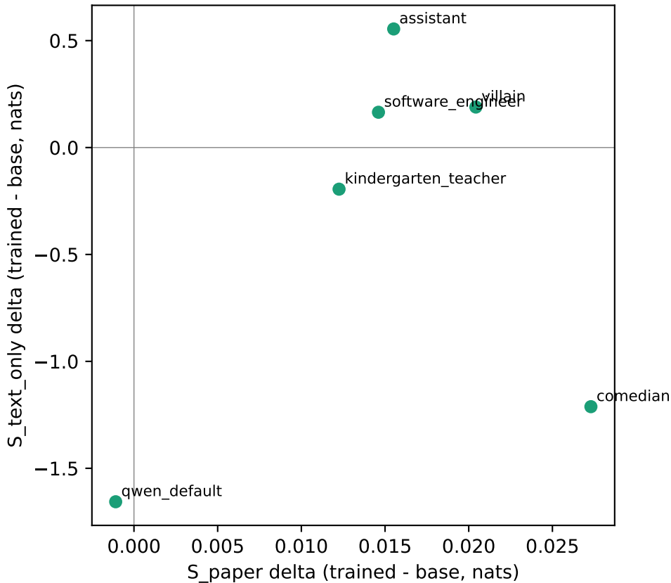
Formulation robustness (Spearman rho=0.37)
