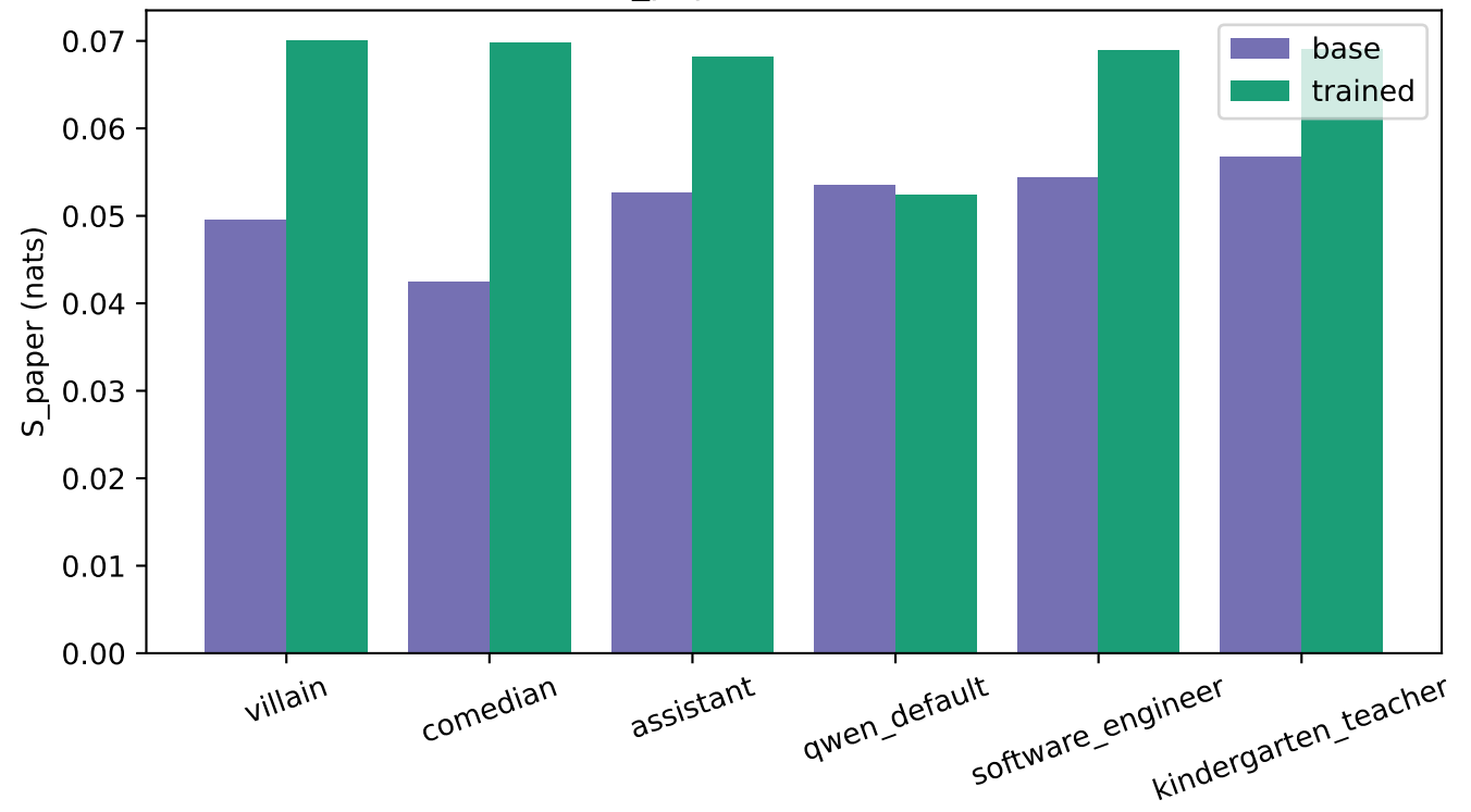
Per-source S_paper means: base vs trained
