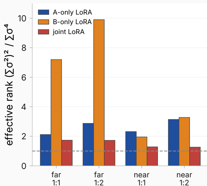
Participation ratio
