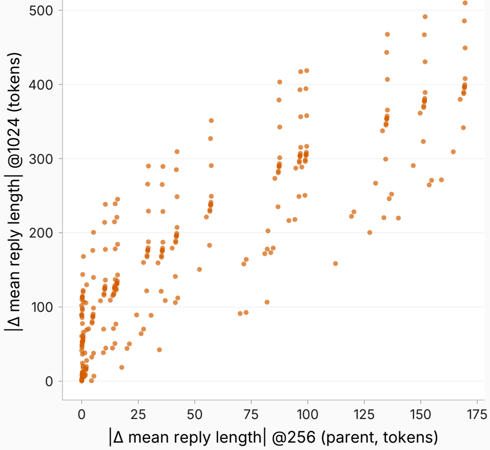
Length feature before vs after the cap lift (per pair)
