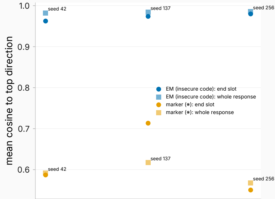
Whole-response vs end-slot read
