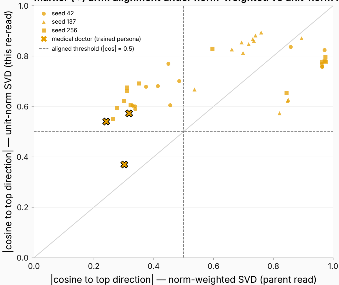
marker (*) arm: alignment under norm-weighted vs unit-norm reads
