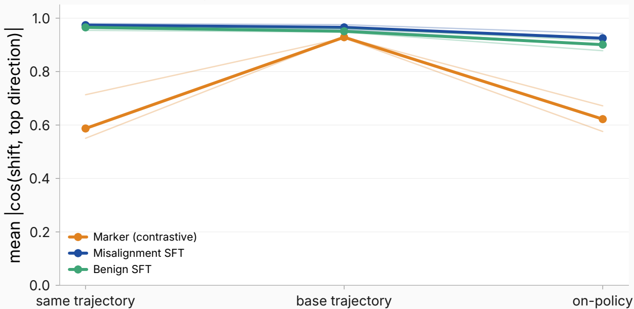
Variant sensitivity of direction concentration (thin = seeds, thick = median)
