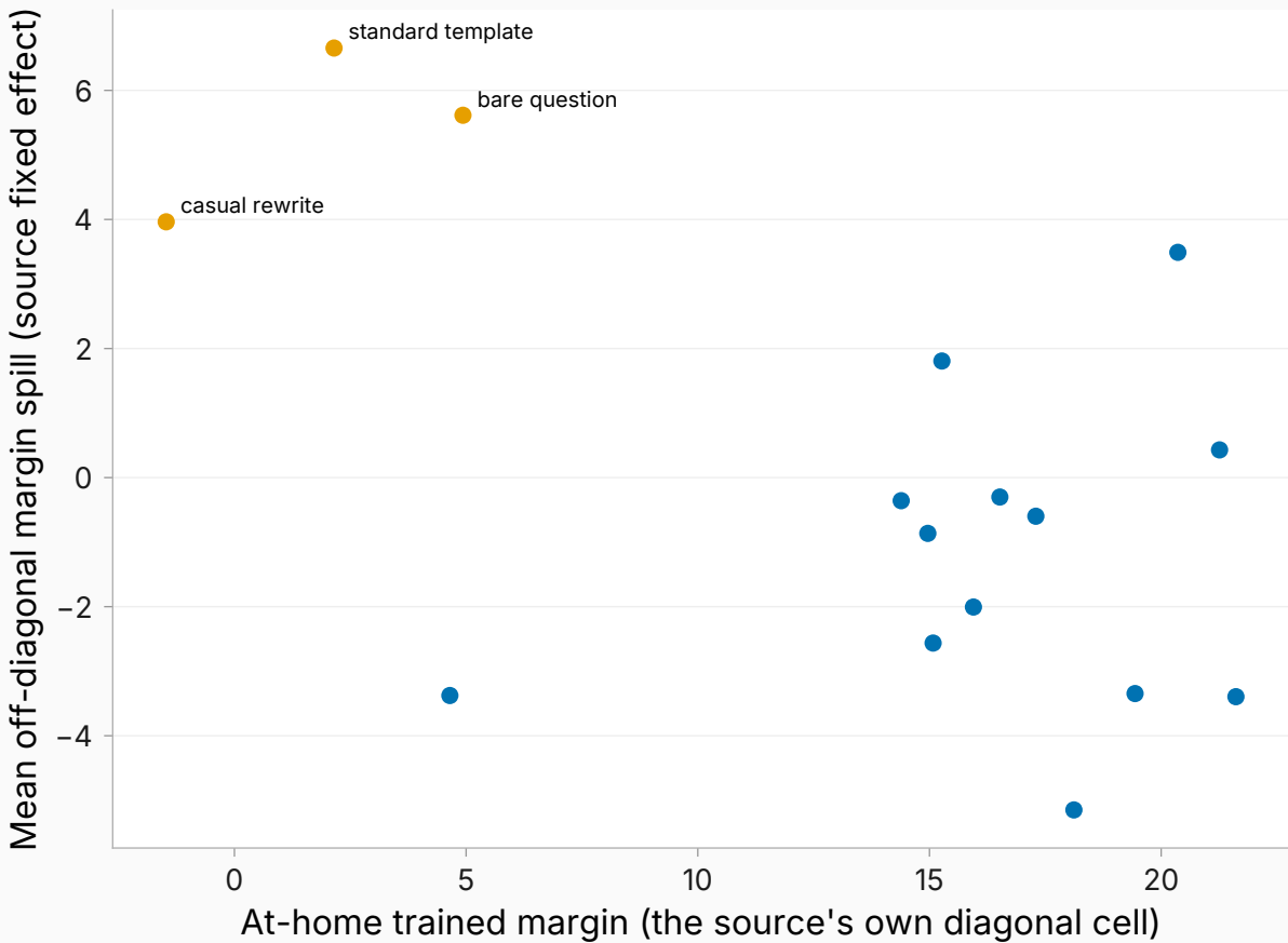
At-home implant strength vs spill onto other contexts, 16 sources (thin prompts highlighted)
