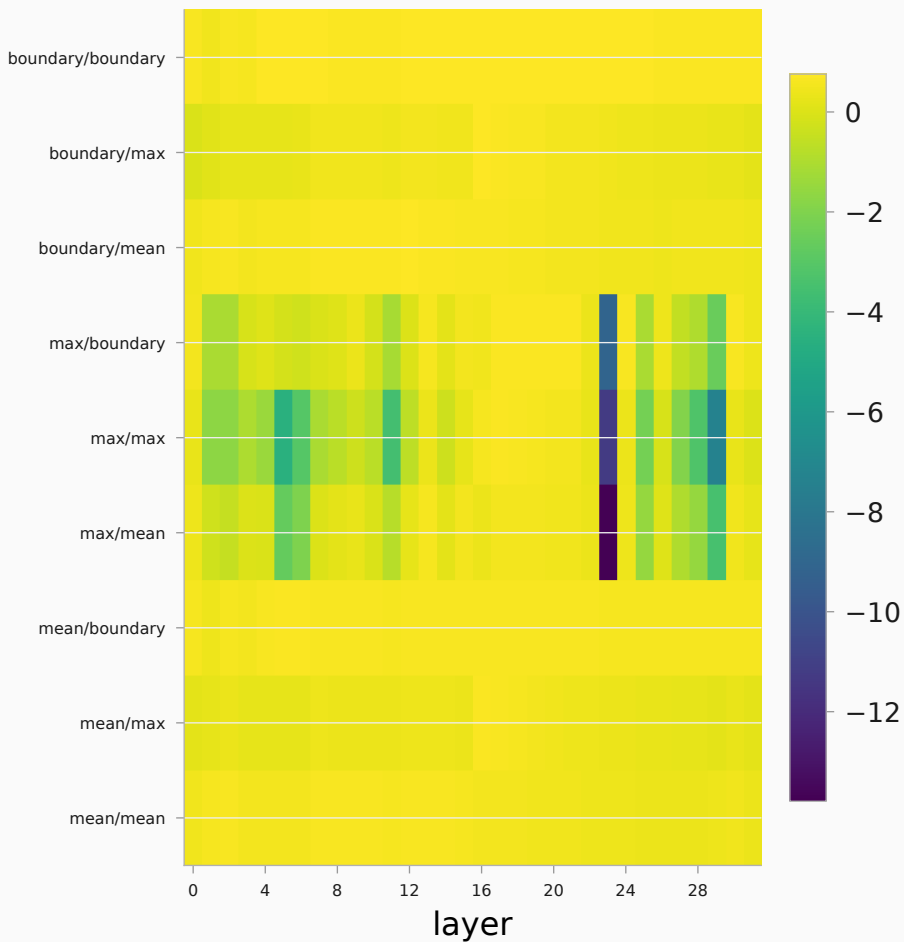
stage 1 (ctx→cot) — LOCO
