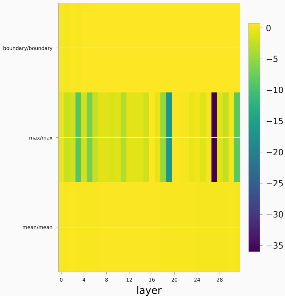
stage 1 (ctx→cot) — LOFO
