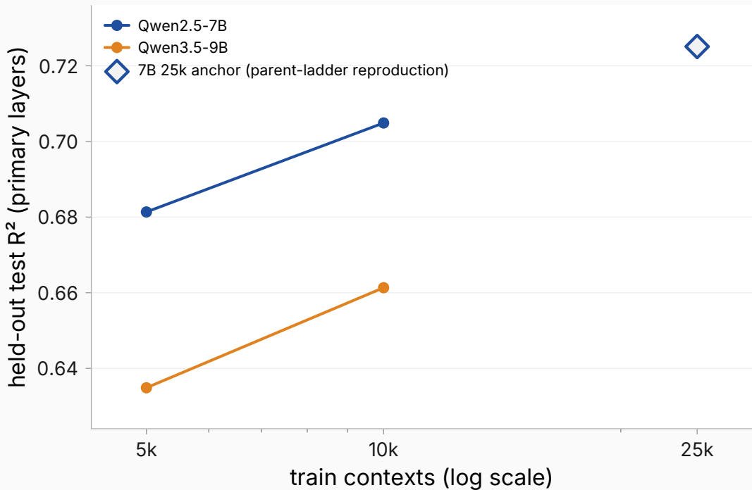
Map R^2 vs train-set size
