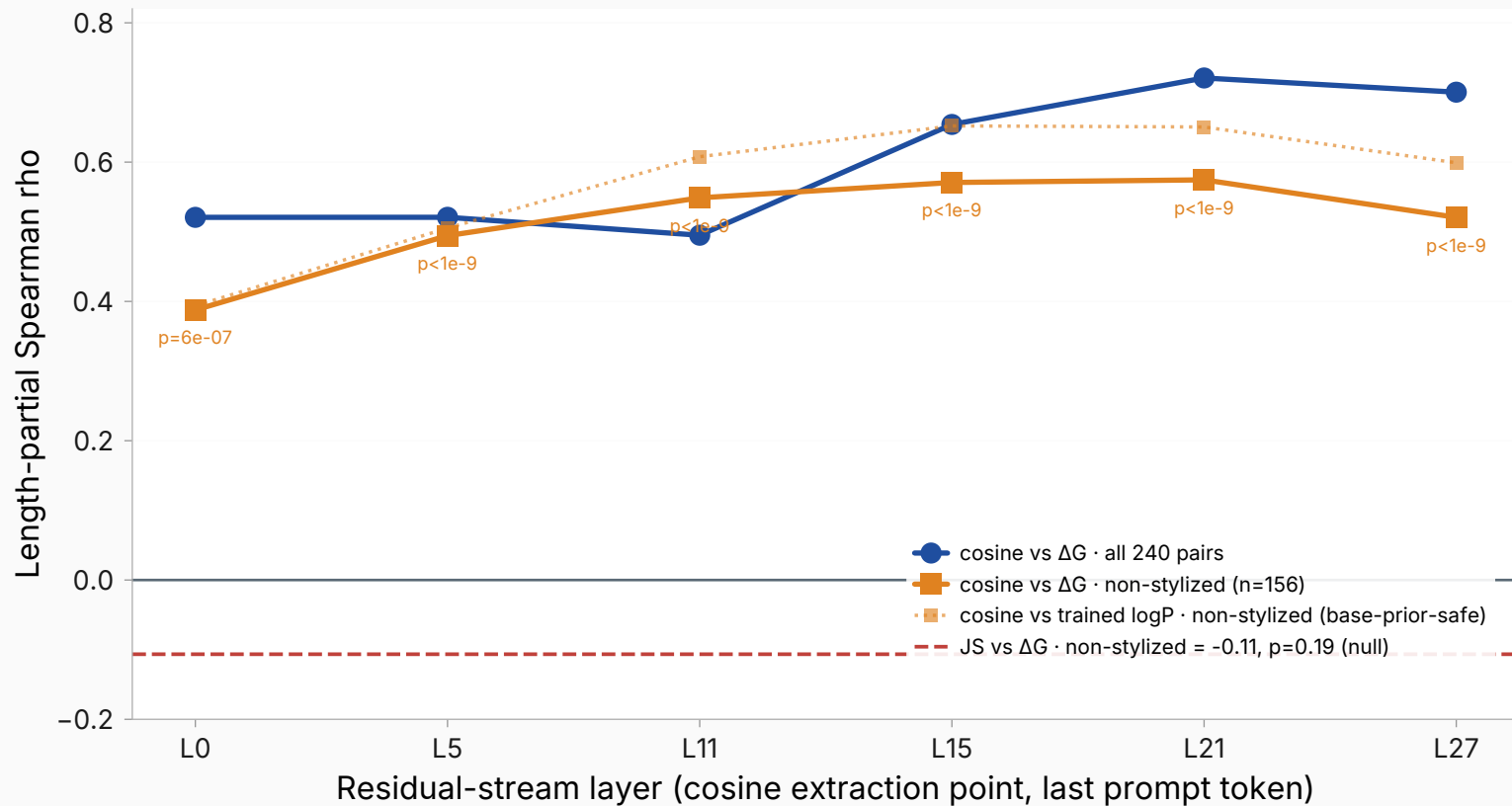
Which layer localizes the transfer-relevant dimension? (localized arm, ep1)
