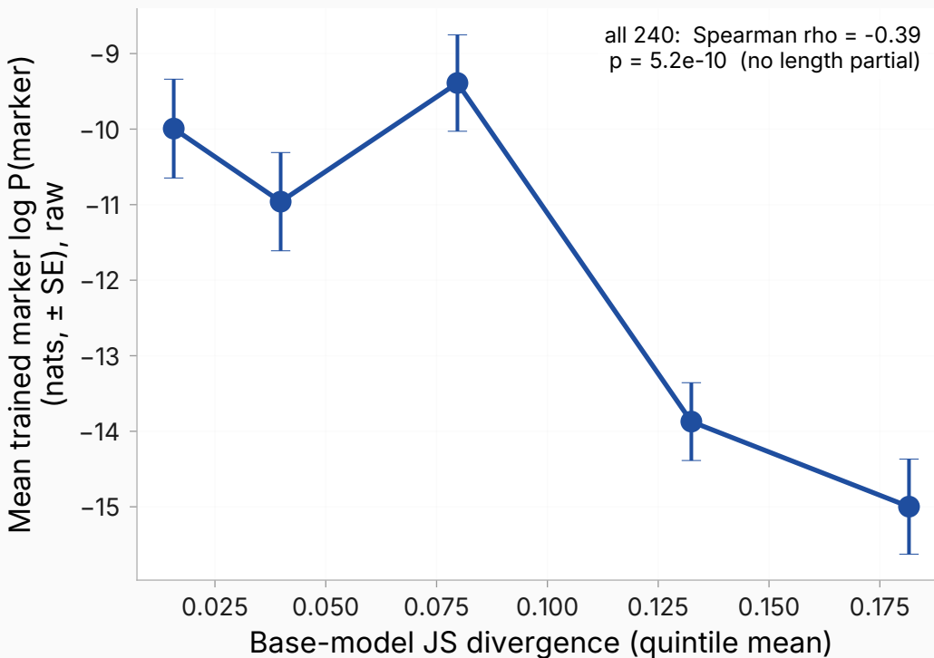
JS divergence \rightarrow lower trained marker log-prob
