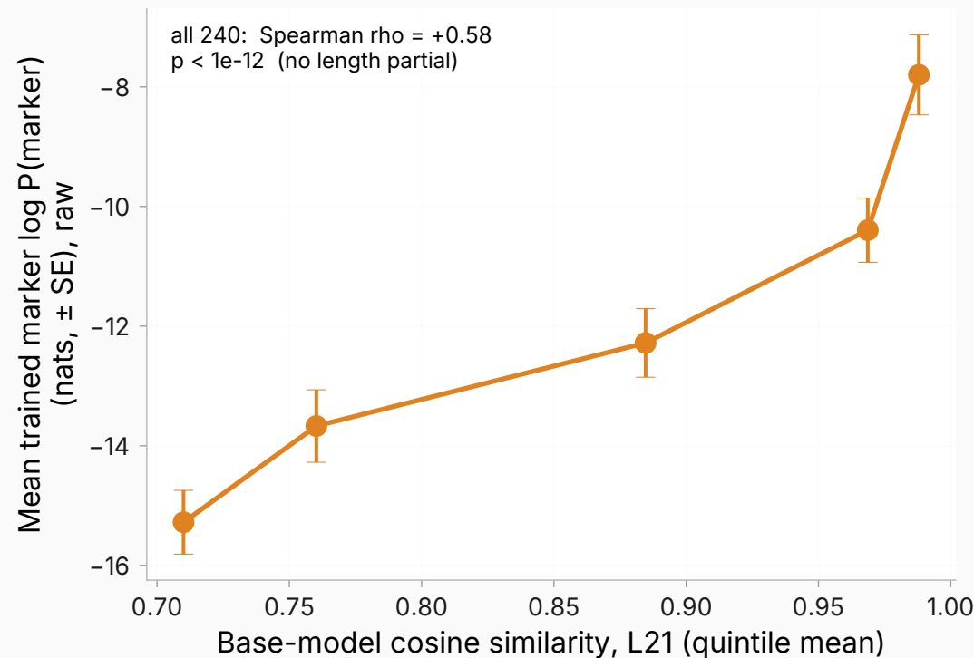
Cosine similarity \rightarrow higher trained marker log-prob
