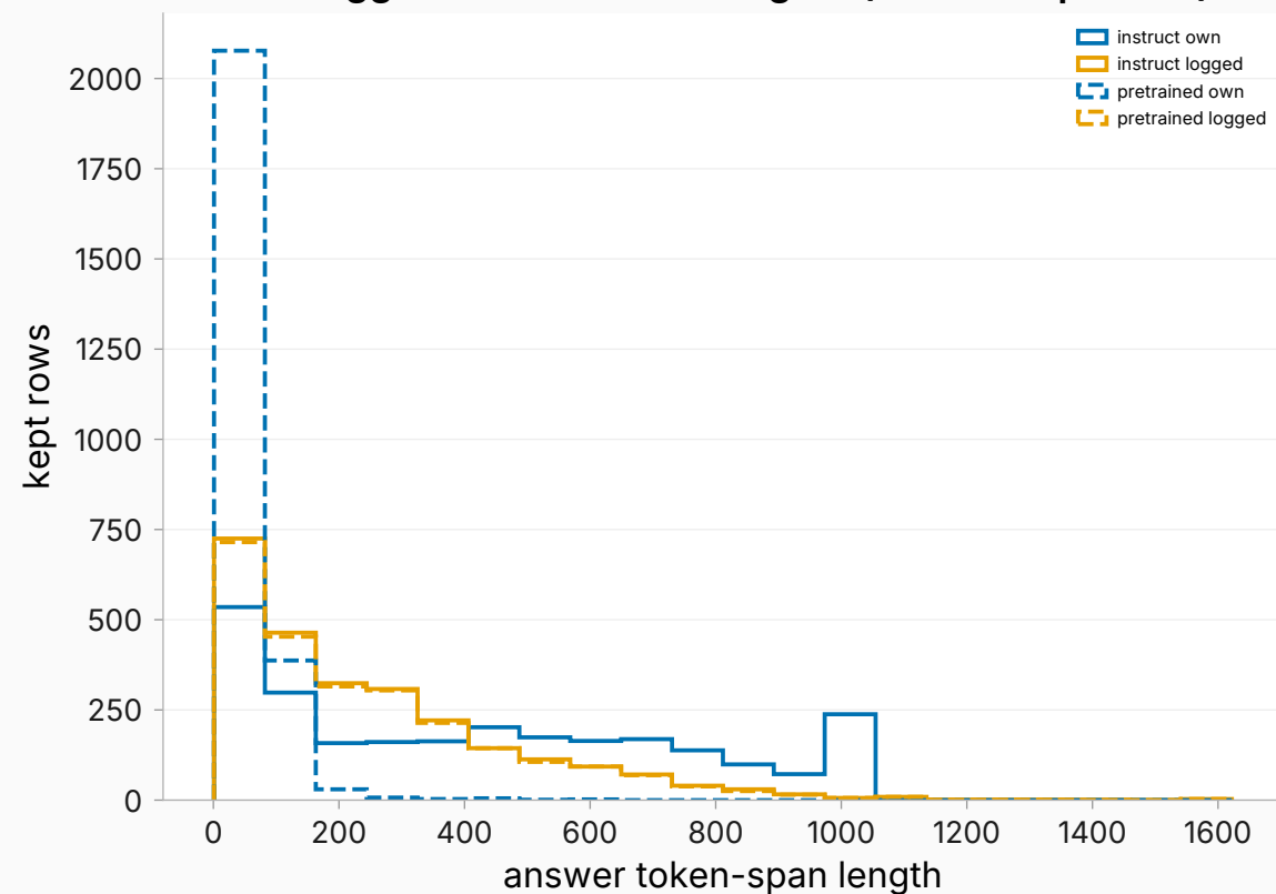
Own vs logged answer token lengths (shared kept rows)
