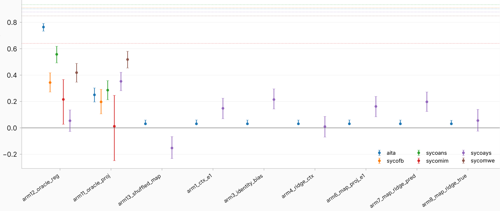
#1739 sycophancy transfer — per-arm rho by eval rung (prefix_end, e1); dotted lines = per-rung split-half ceilings
