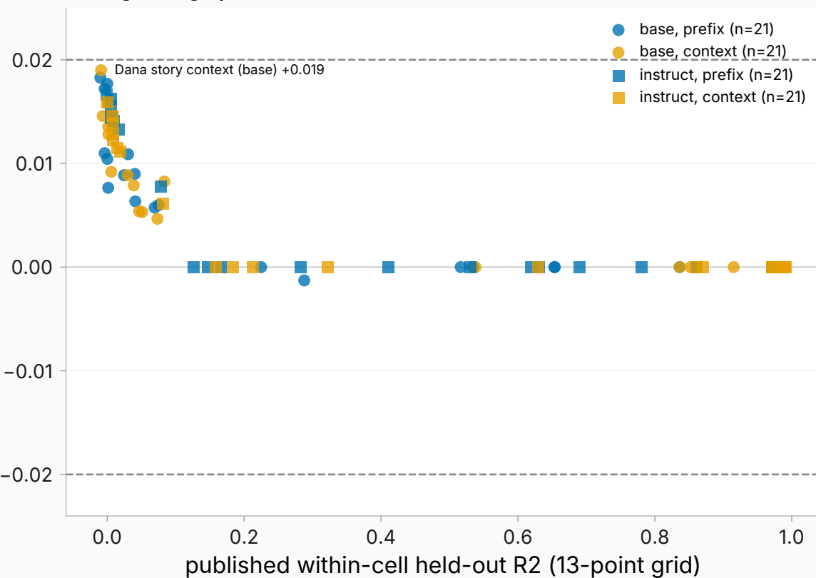
ceiling change per cell-arm (84 of 84 inside the 0.02 bar)
