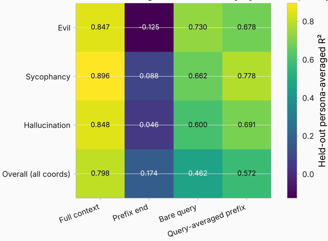
Persona-averaged trait readability by arm (L14, 996 prefixes)
